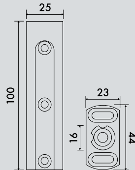
Track & Slide M 100 kg
