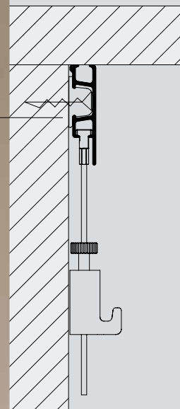
Click Rail Pro
