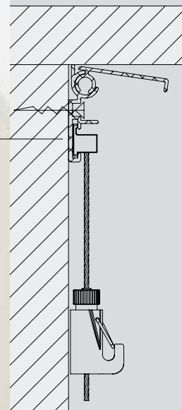
Double Wall Track
