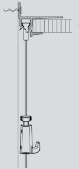
Shadowline Masonry
